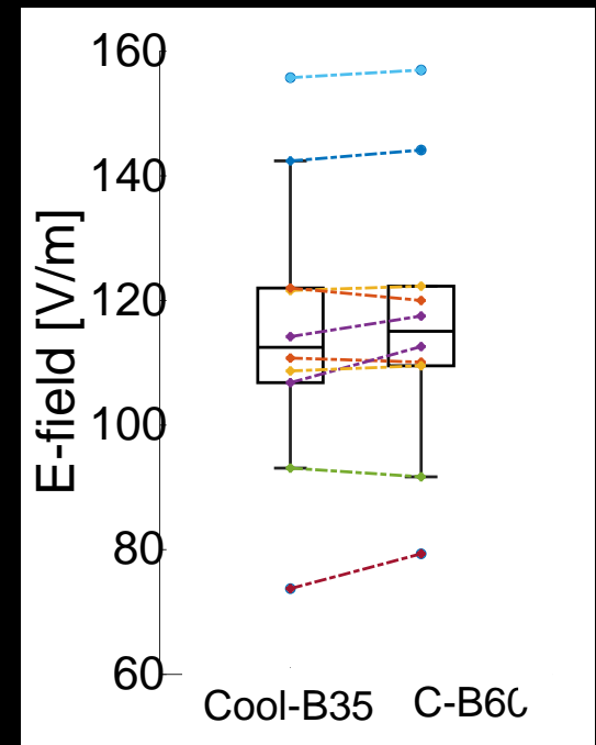
Peak E-field on motor area
